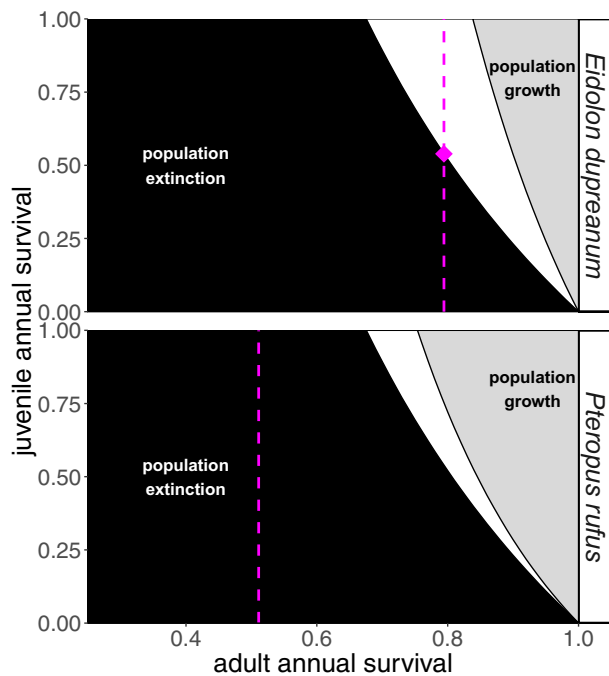
Fig. 2. Zero-growth isoclines for Madagascar's fruit bats.
