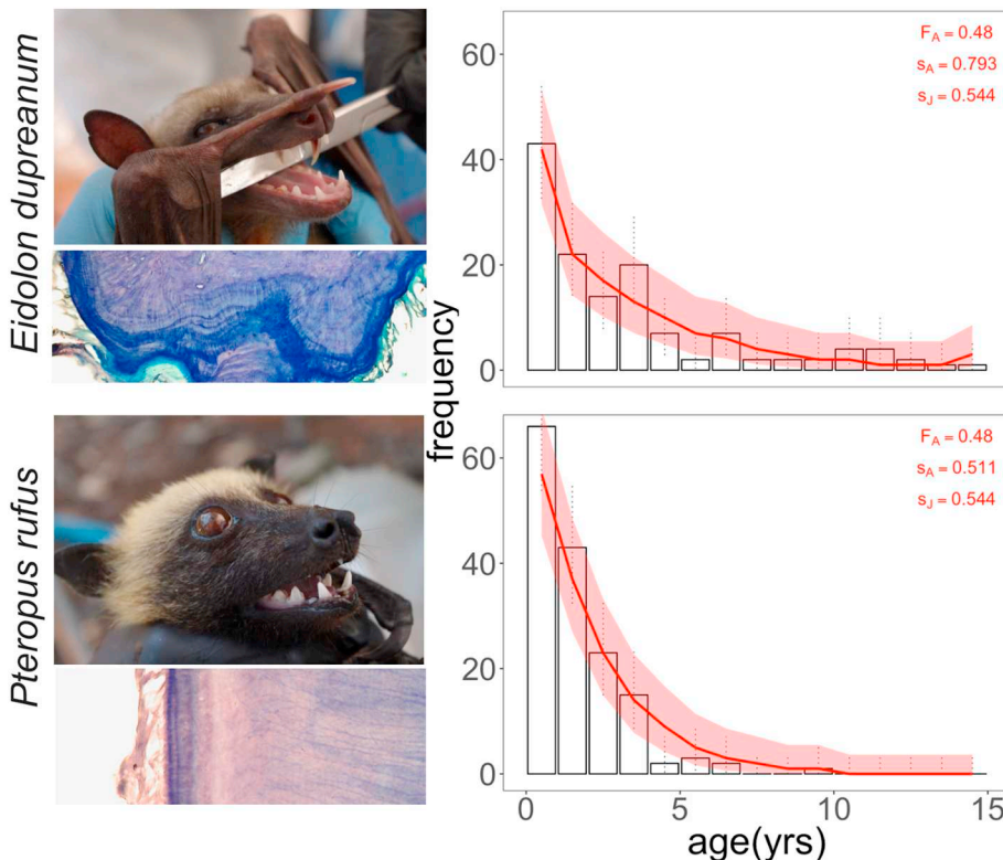
Fig. 1. Age-frequency data and fitted survival models for Madagascar's fruit bats.
