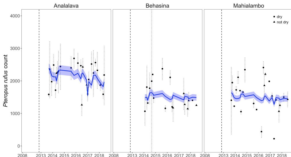
Fig. 3. Longitudinal exit counts for three Pteropus rufus roosts in the District of Ambatondrajaka, Madagascar.
